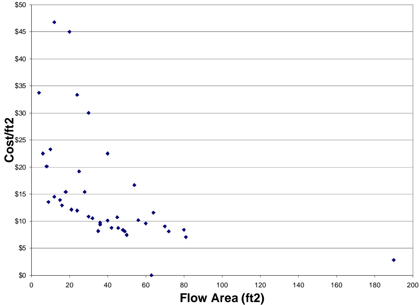
Figure C-1. Cost per Square Foot of Flow Area vs. Flow Area of Culverts
