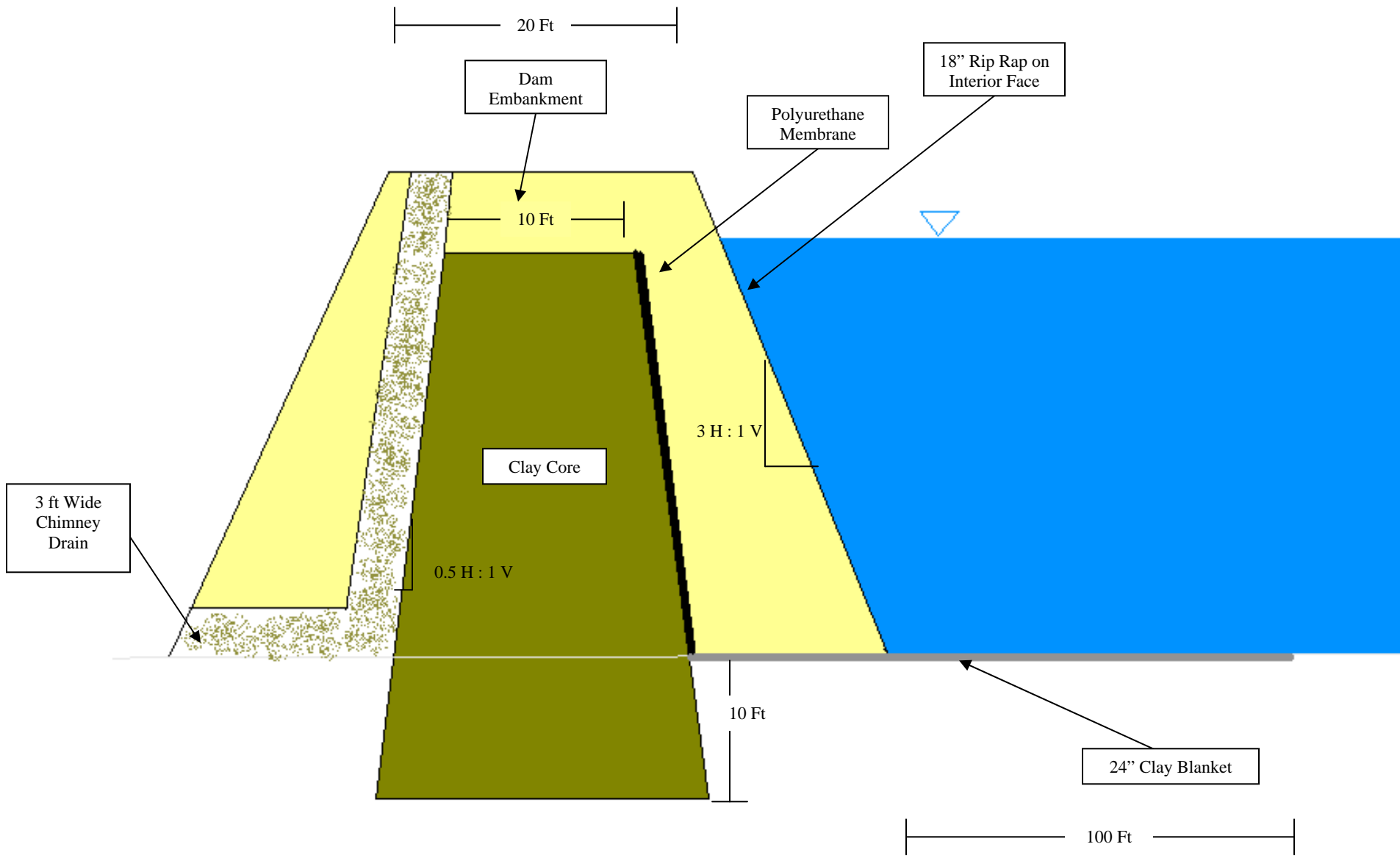
Figure C-2. URS Basin Conceptual Design Embankment Stabilization Materials
