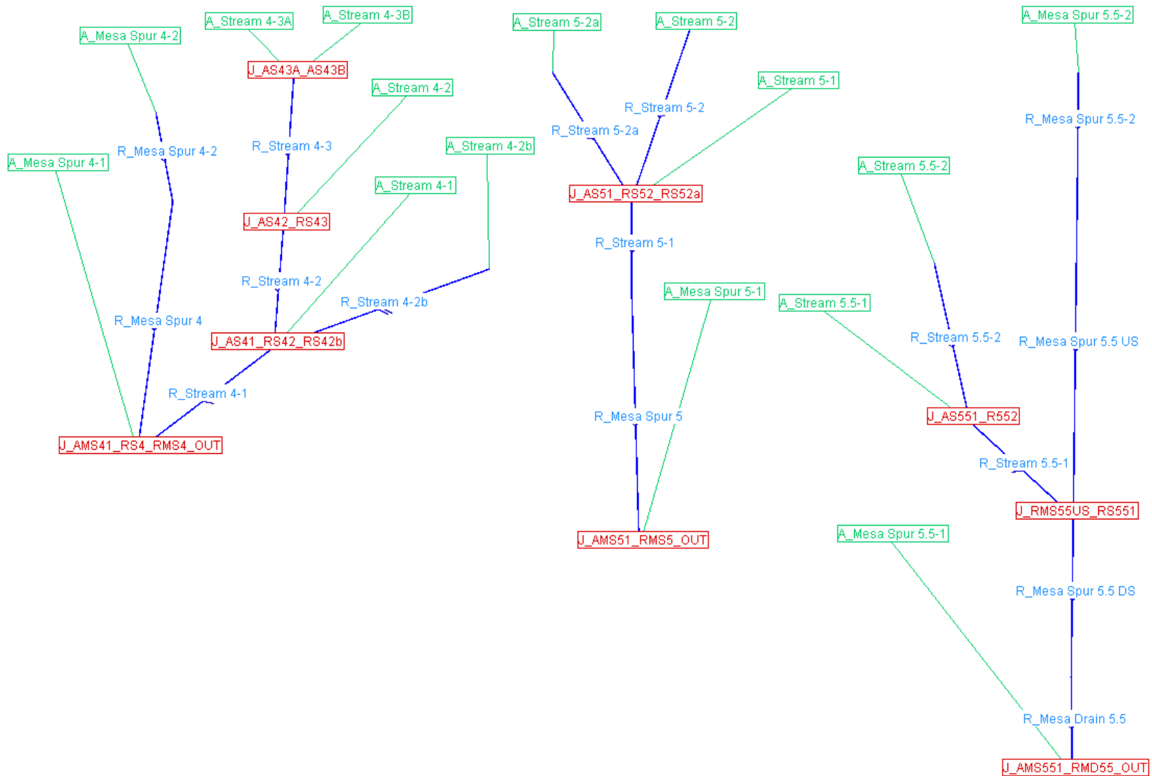
Figure A-36. HEC-HMS Model Layout – Socorro Study Area
