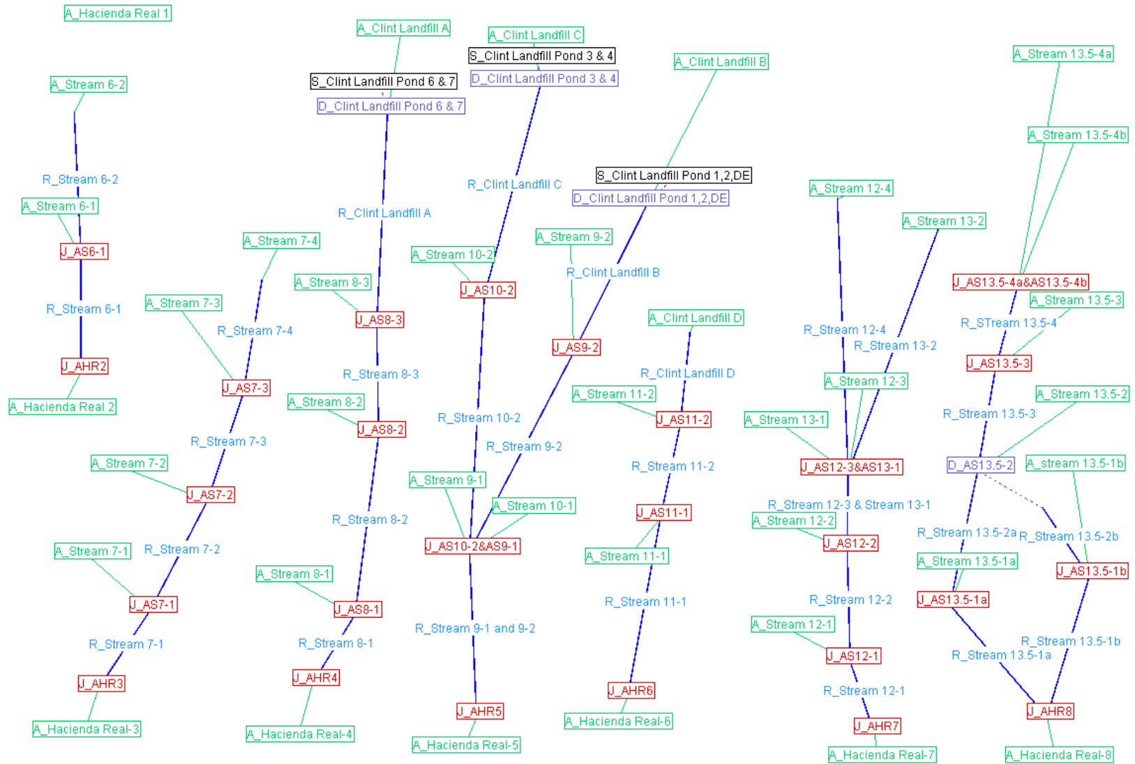
Figure A-37. HEC-HMS Model Layout – Hacienda Real Study Area
